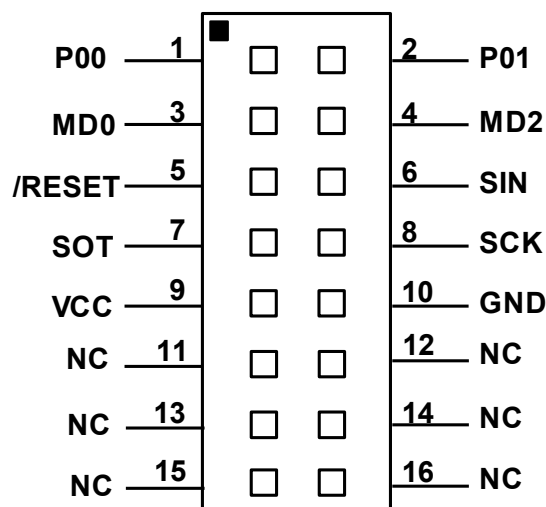
Drawing 1: SYNC connector of ISP-adapter
