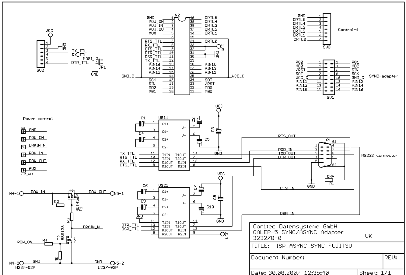
Illustration 4: Schematic of ISP-ASYNC/SYNC adapter 210915
