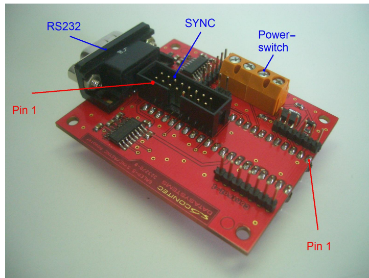
Illustration 1: ISP-ASYNC/SYNC-adapter 210915
