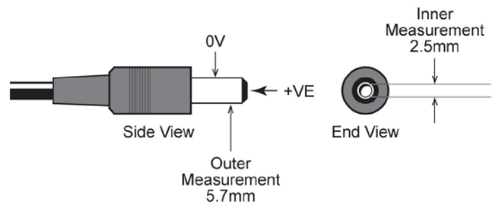
2.5mm Barrel (Jack) Plug
